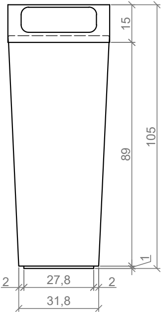
ALZADO / FRONT VIEW
