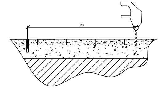
perforar 2 agujeros a una distancia de 165 cm drill 2 holes each other at a distance of 165 cm
