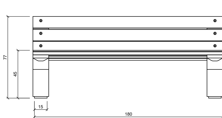
ALZADO / FRONT VIEW
