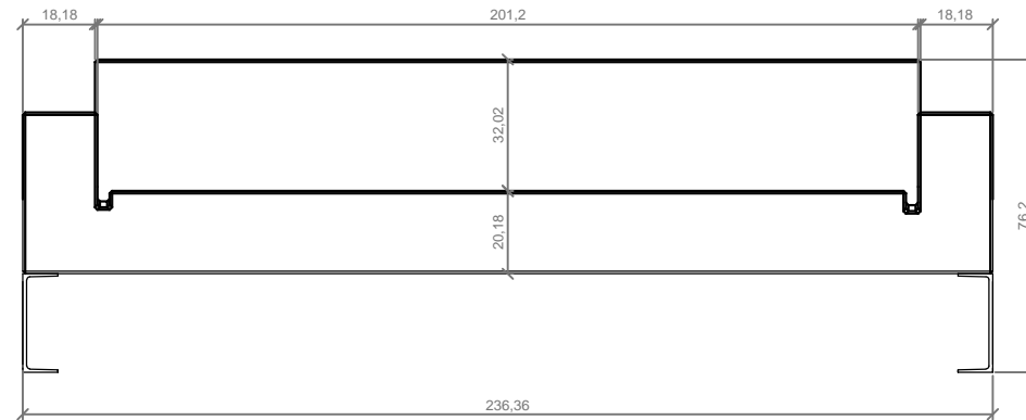
ALZADO / FRONT VIEW
