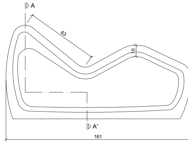
ALZADO / FRONT VIEW
