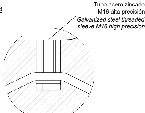
DETALLE C / DETAIL C
