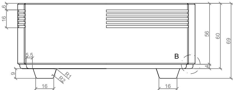
VISTA INFERIOR / BOTTOM VIEW
