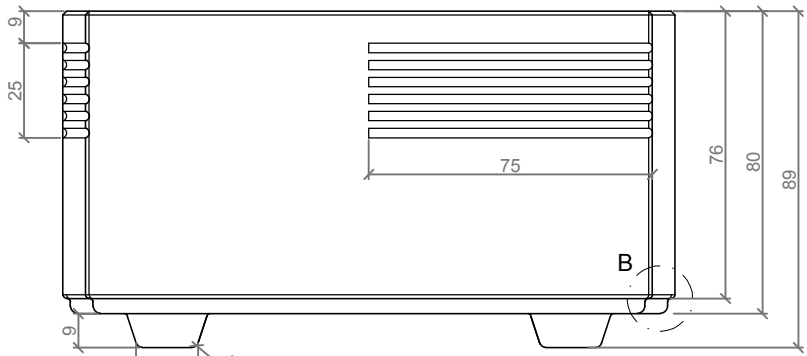
VISTA INFERIOR / BOTTOM VIEW
