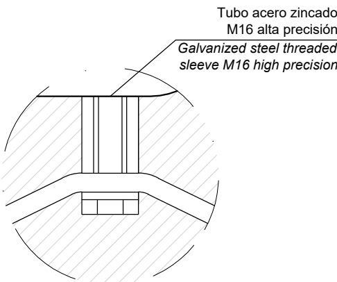
DETALLE C / DETAIL C
