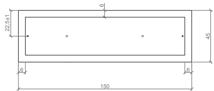
VISTA INFERIOR / BOTTOM VIEW
