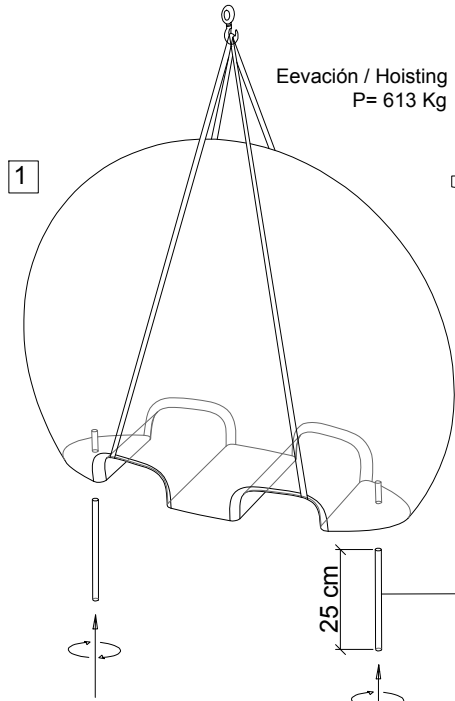
Varilla roscada Ø16 Threaded rod Ø16
