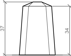
ALZADO / FRONT VIEW
