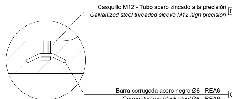
DETALLE D / DETAIL D
