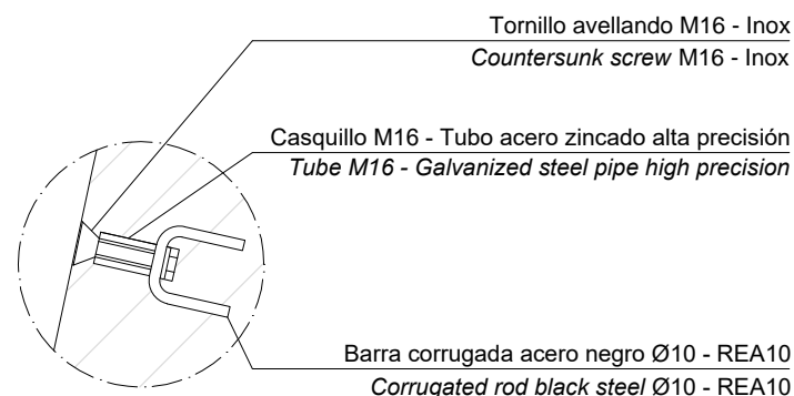
DETALLE / DETAIL
