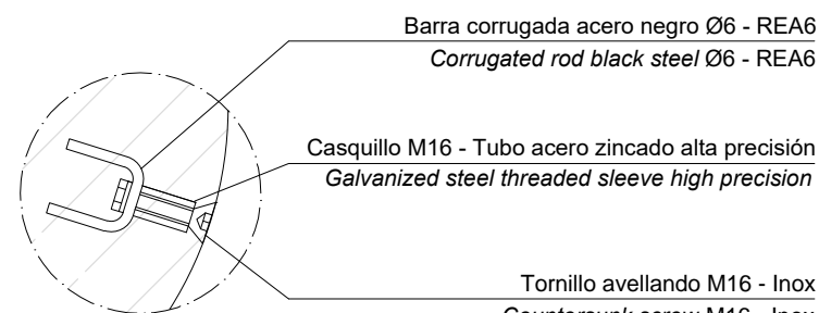
DETALLE / DETAIL
